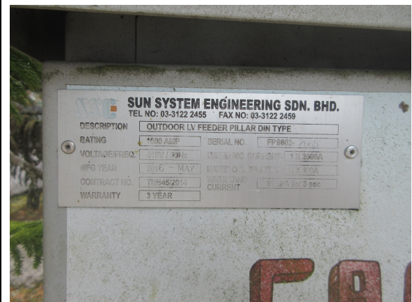
FEEDER PILLAR TX2 NAMEPLATE
