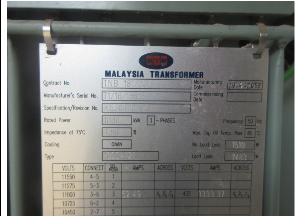
TRANSFORMER 2 NAMEPLATE
