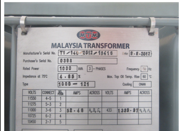
TRANSFORMER 1 NAMEPLATE
