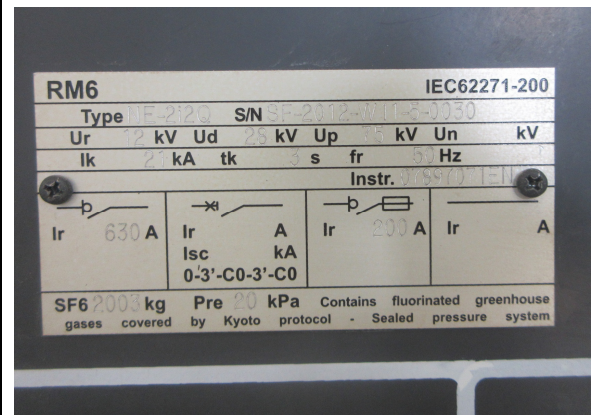
SWITCHGEAR NAMEPLATE
